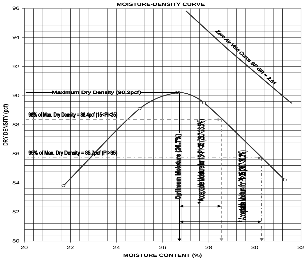
PLOT OF SAMPLE MOISTURE-DENSITY CURVE * Acceptance limits based on 2004 Item 132 Specifications
